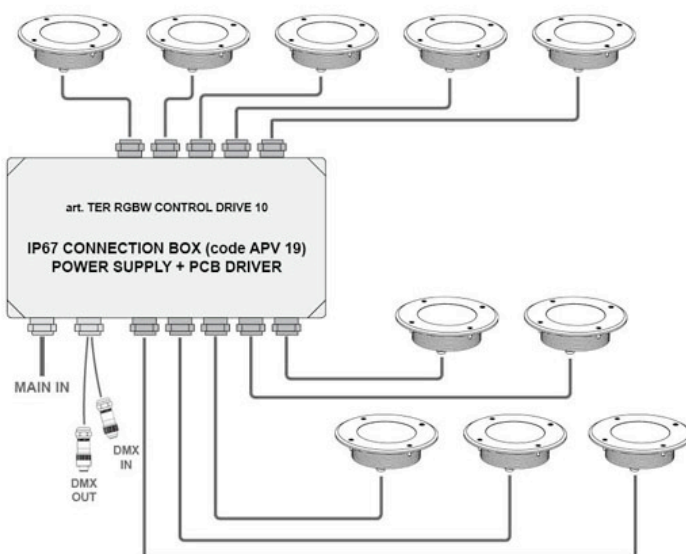
Example of RGBW connection up to 10 fixtures
